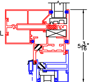
5 HORIZONTAL TDL
