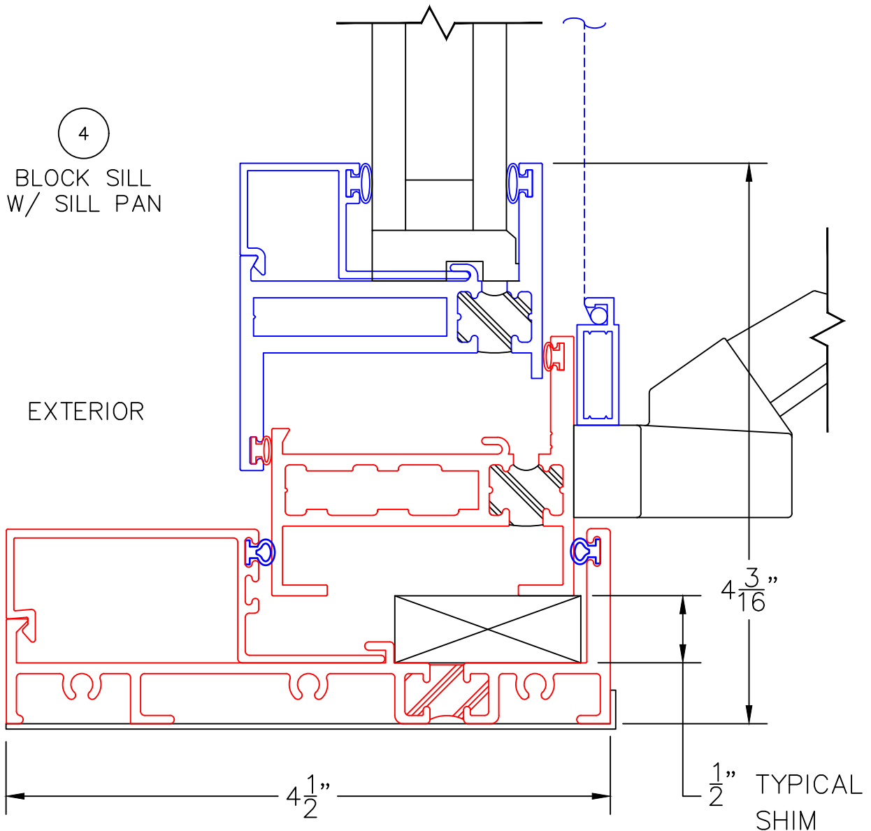
3800-T SILL WITH 350-T AWNING INSERT
