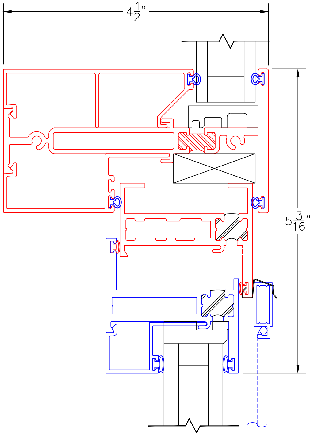
3800-T 1" GLAZING OVER 350-T AWNING INSERT
