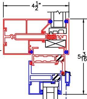
3 HORIZONTAL TDL
