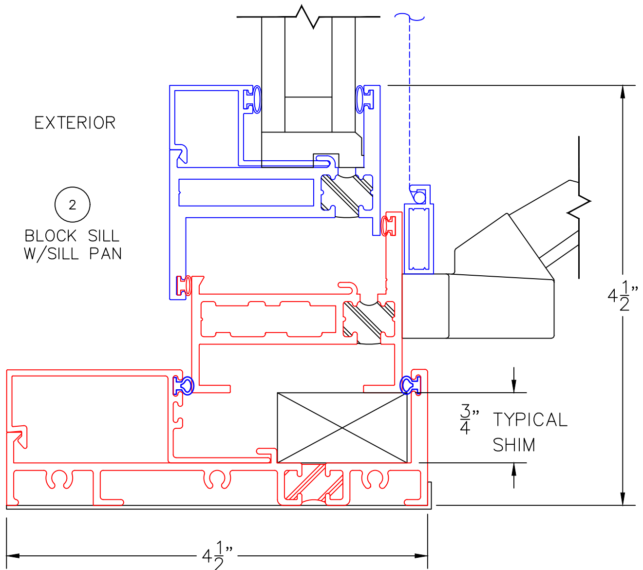
3800-T SILL WITH 350-T CASEMENT INSERT
