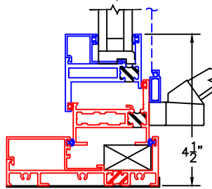
2 BLOCK SILL W/ SILL PAN
