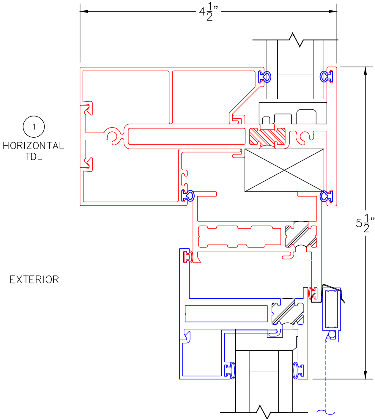
3800-T 1" GLAZING OVER 350-T CASEMENT INSERT
