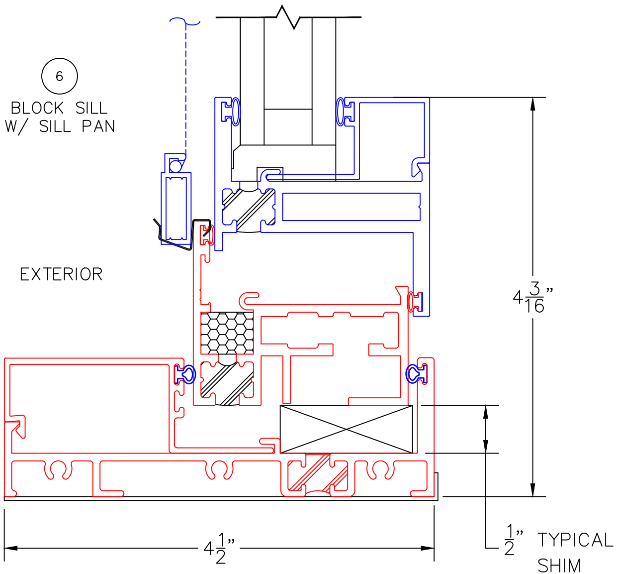
3800-T SILL WITH 350-T HOPPER INSERT
