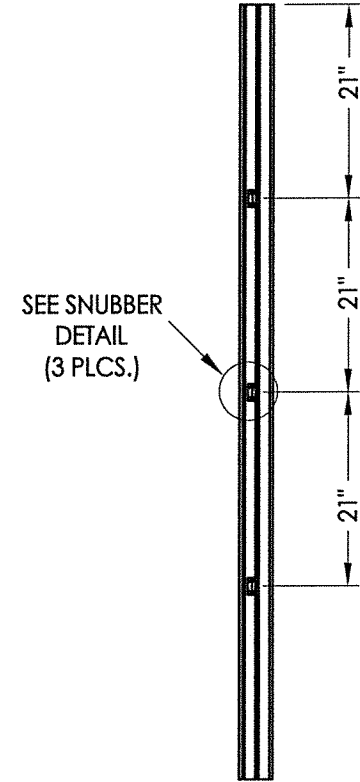
SNUBBERS JAMB
