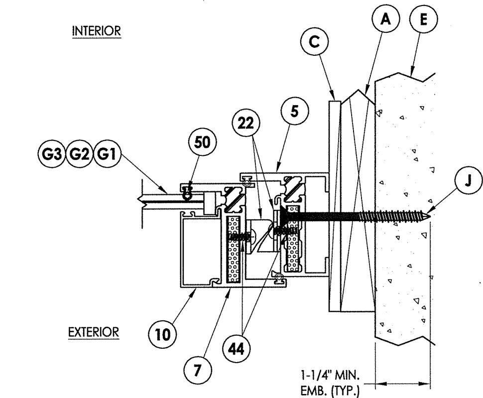
2 HORIZONTAL CROSS SECTION 3 Shown w/ 1X Sub buck option
