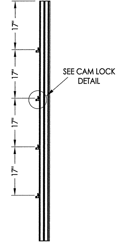
LOCK JAMB CAM LOCKING POINTS (4)
