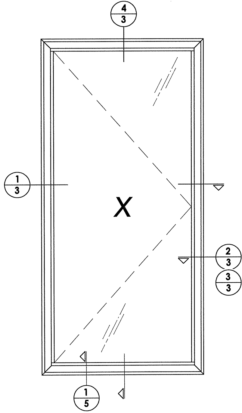
4-BAR HINGE
