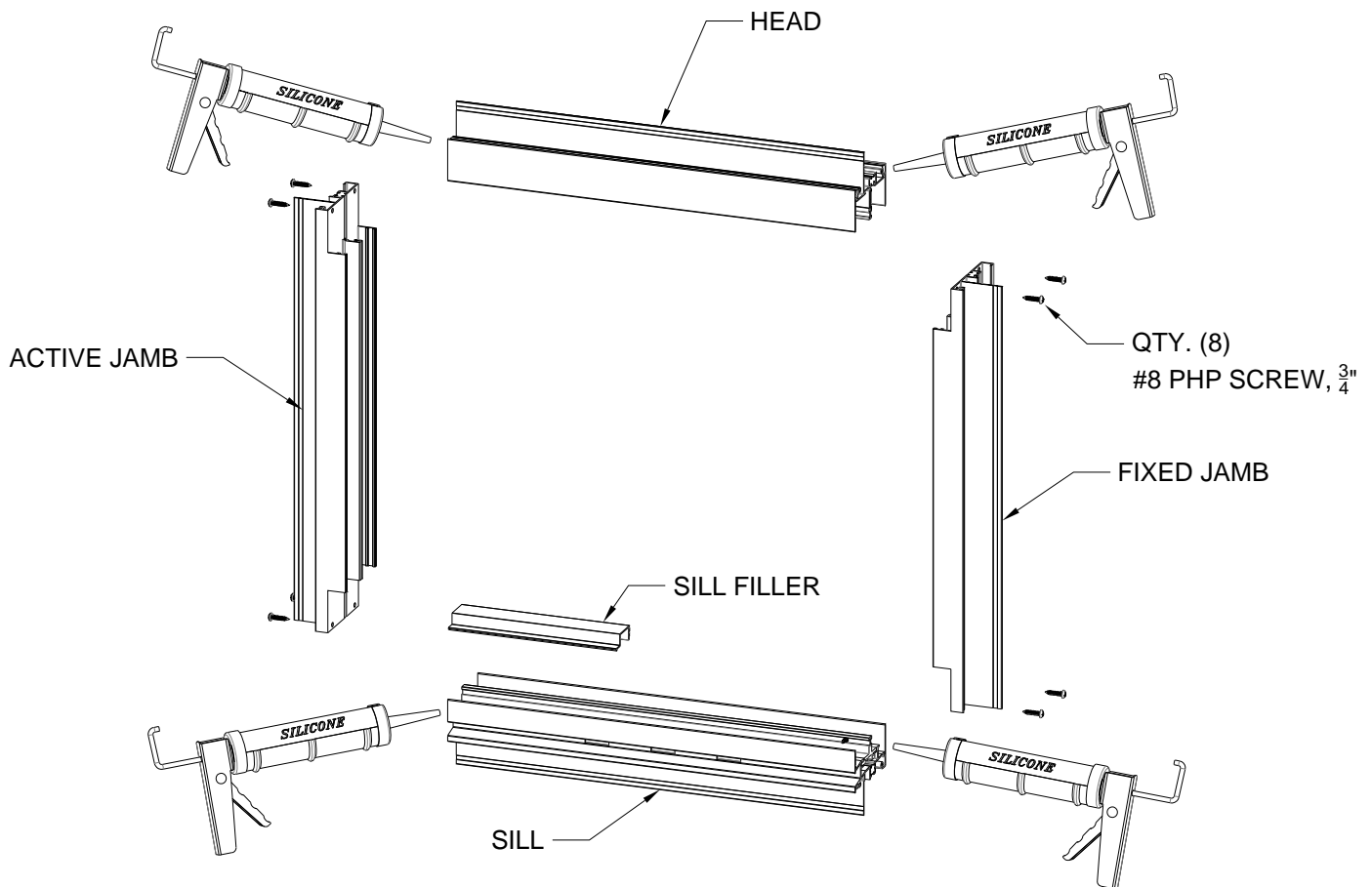
Figure 10: Frame Assembly
