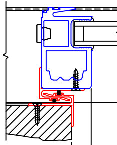
④ L-TYPE POCKET INTERLOCKER WITH REVERSE HP INTERLOCKER
