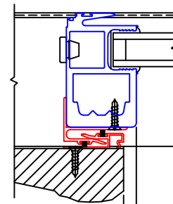
⑤ J-POST POCKET INTERLOCKER WITH REVERSE HP INTERLOCKER
