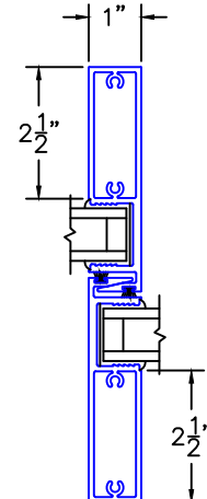
⑧ NARROW HP INTERLOCKERS (BOTH SIDES)
