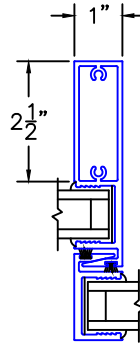
⑦ NARROW HP INTERLOCKERS (INTERIOR SHOWN)
