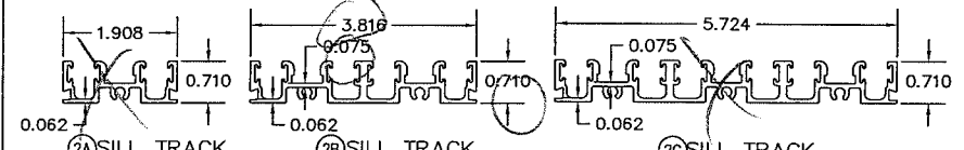
(2A) SILL TRACK SINGLE RUN (2B) SILL TRACK DOUBLE RUN (2C) SILL TRACK TRIPLE RUN
