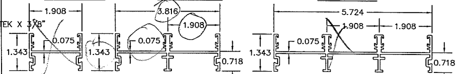
(3A) SIDE TRACK SINGLE RUN (3B) SIDE TRACK DOUBLE RUN (3C) SIDE TRACK TRIPLE RUN
