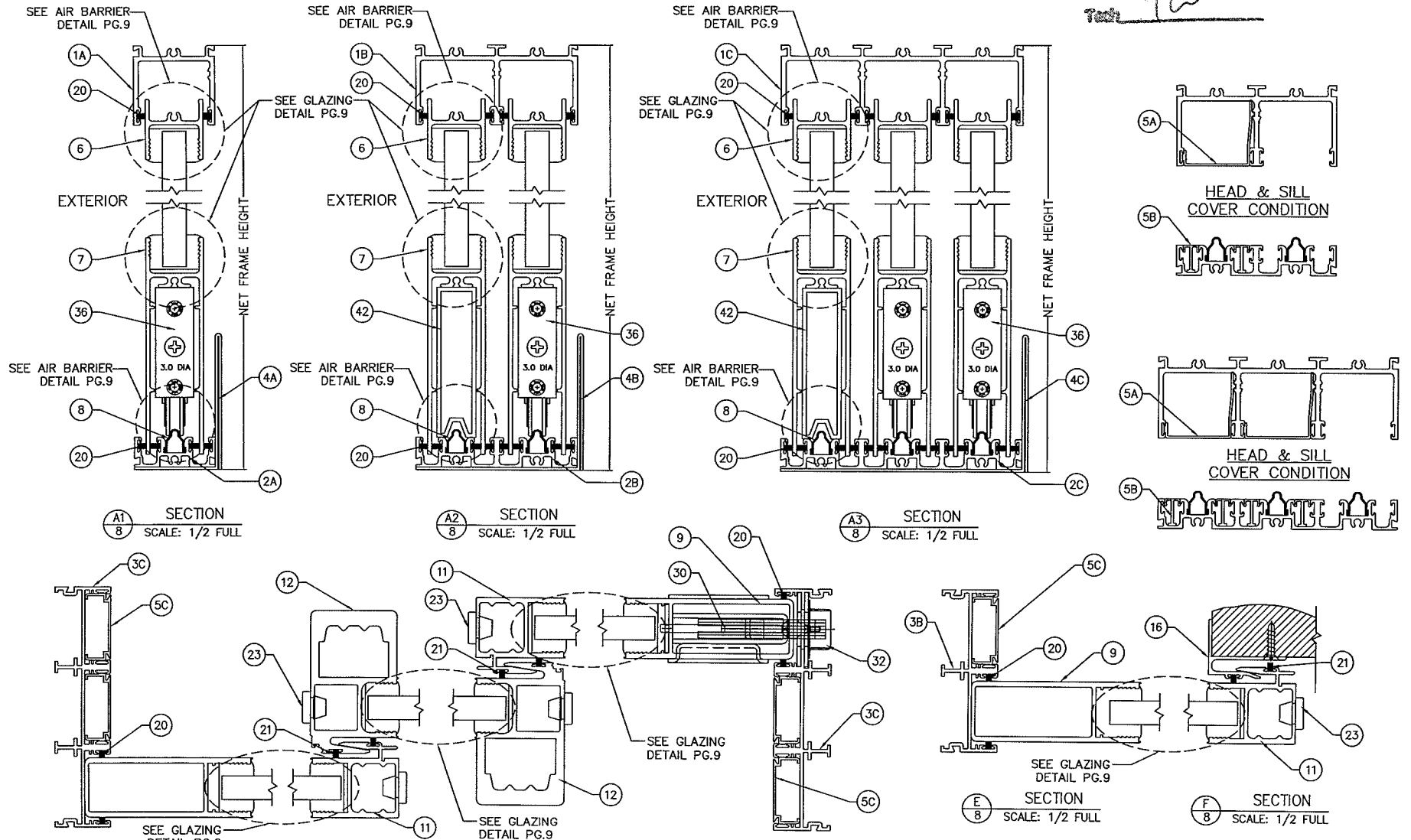
B SECTION SCALE: 1/2 FULL
