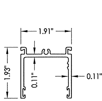
21 HEAD TRACK 1 Run
