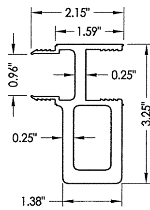
13 WINDLOAD ADAPTER
