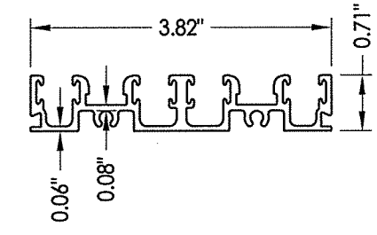
2 SILL TRACK 2 Runs
