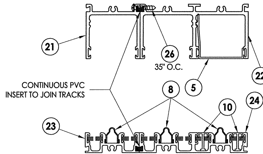
HEAD & SILL COVER CONDITION
