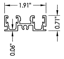
23 SILL TRACK 1 Run
