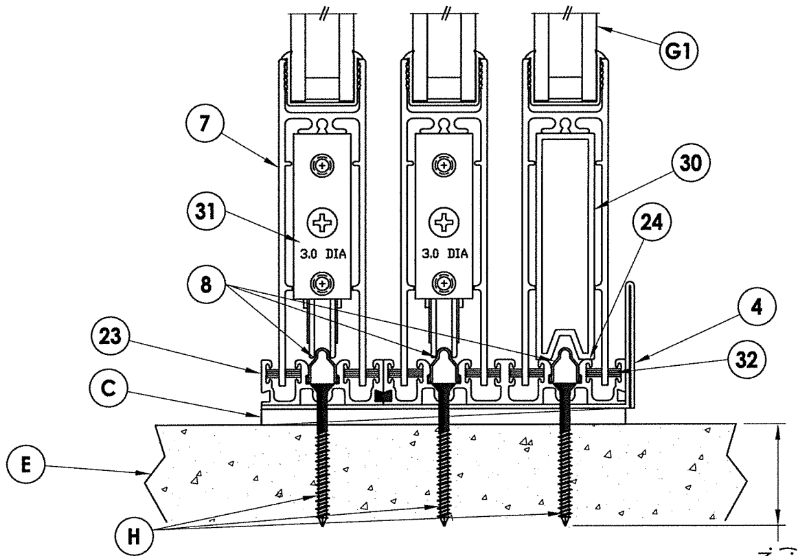
2 VERTICAL CROSS SECTION 3 Direct to masonry
