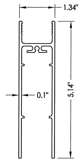
7 BOTTOM RAIL
