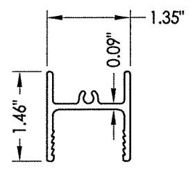
6 TOP RAIL
