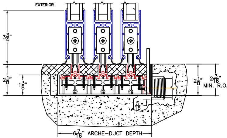
2 1" SIDE DRAIN TO INTERIOR (OPT-D1)
