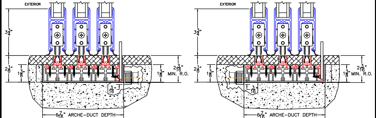
2 1/2" SIDE DRAIN TO INTERIOR (OPT-D2)
