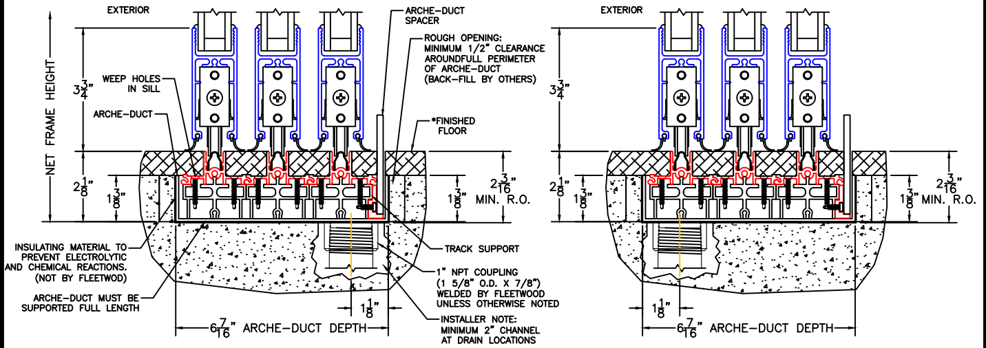
1 1" BOTTOM DRAIN TO INTERIOR (OPT-A)
