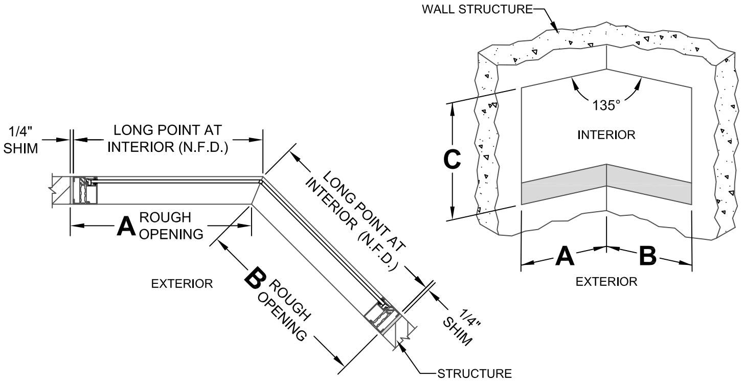
PLAN VIEW SERIES 350-T SHOWN
