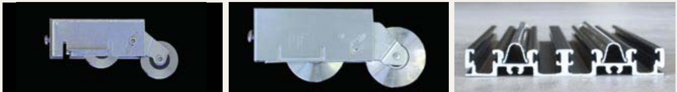
S.S. Precision Roller – 1.812" diameter (Norwood 3000, Glacier 3300 & Oasis 3033) Mammoth S.S. Precision Roller – 3" diameter (Norwood 3050, 3070-EX, CR, HI-WG) S.S. Track Insert
