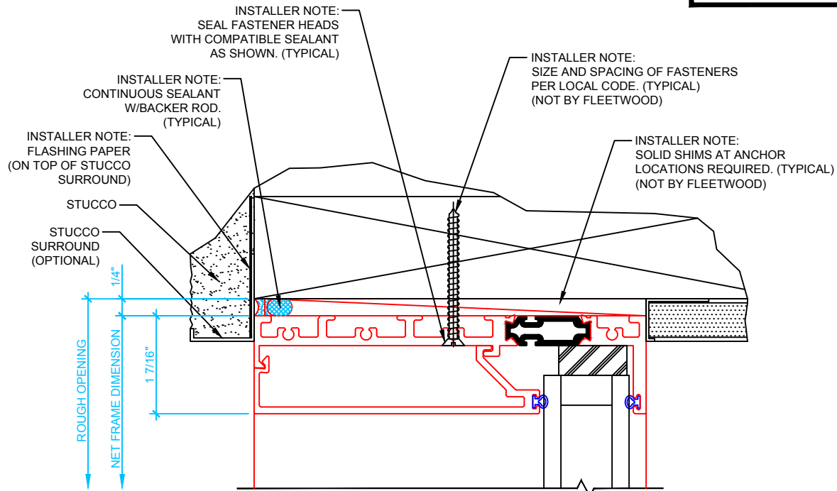
EXTERIOR 1 FIXED WINDOW HEAD JAMBS SIMILAR SCALE: 6" = 1'
