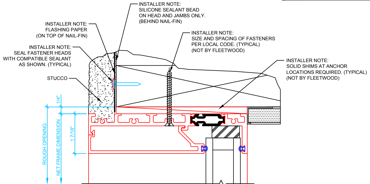
EXTERIOR 1 FIXED WINDOW HEAD JAMBS SIMILAR SCALE: 6" = 1'
