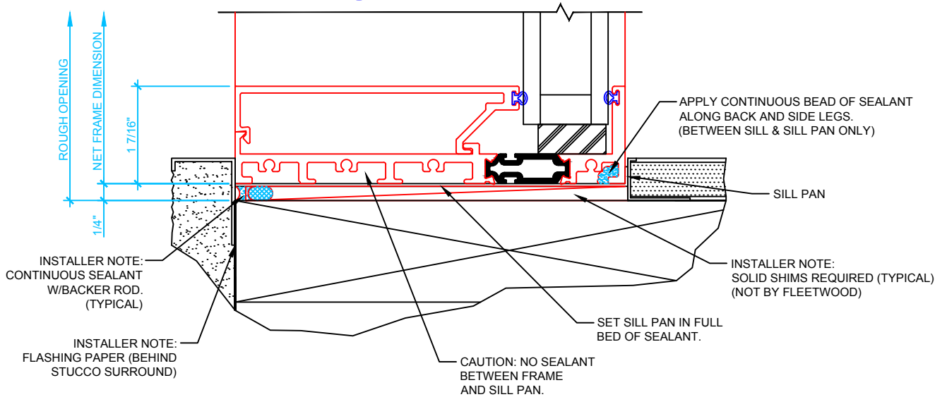
EXTERIOR 1 FIXED WINDOW HEAD JAMBS SIMILAR SCALE: 6" = 1'
