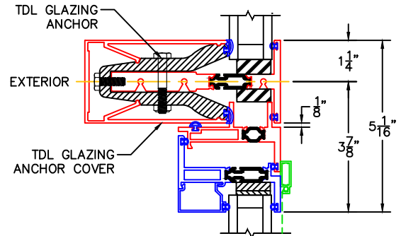
3 HORIZONTAL TDL WITH FIXED OVER CSMNT/AWNG INSERT
