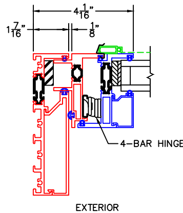
5 BLOCK JAMB WITH AWNING INSERT
