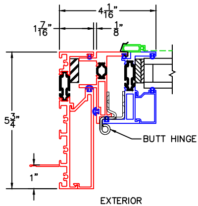
4 NAIL-FIN JAMB WITH CASEMENT INSERT
