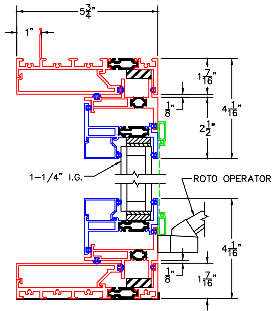
1 NAIL-FIN HEAD W/CSMNT/AWNG INSERT
