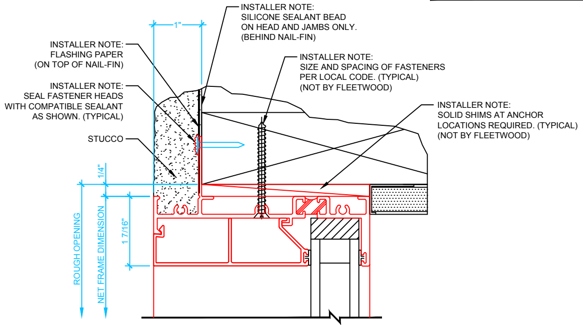
EXTERIOR 1 FIXED WINDOW HEAD JAMBS SIMILAR SCALE: 6" = 1'
