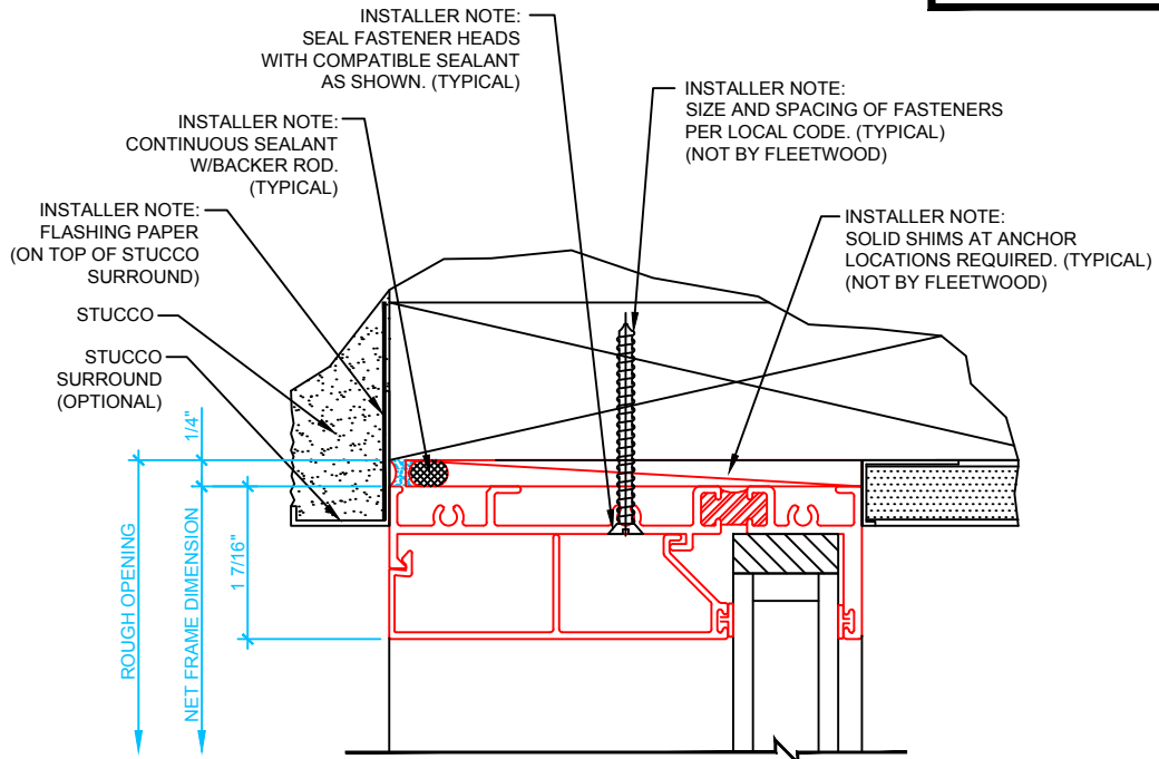
EXTERIOR 1 FIXED WINDOW HEAD JAMBS SIMILAR SCALE: 6" = 1'
