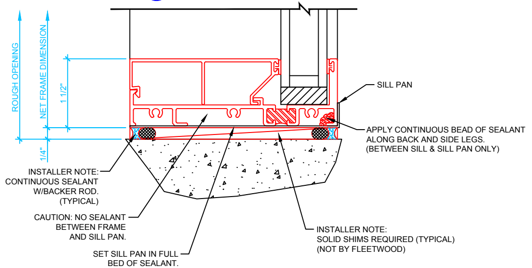
EXTERIOR 1 FIXED WINDOW HEAD JAMBS SIMILAR SCALE: 6" = 1'
