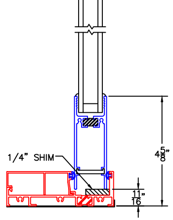
3B BLOCK JAMB W/ARCHETYPE STILE INSERT
