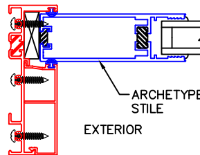
4B VERTICAL TDL W/ARCHETYPE STILE INSERT
