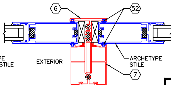
4B VERTICAL TDL W/ARCHETYPE STILE INSERT
