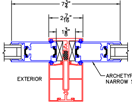
4A VERTICAL TDL W/ARCHETYPE NARROW STILE INSERT
