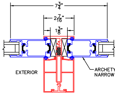
4A VERTICAL TDL W/ARCHETYPE NARROW STILE INSERT
