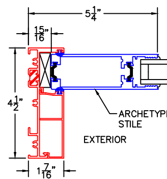
4B VERTICAL TDL W/ARCHETYPE STILE INSERT
