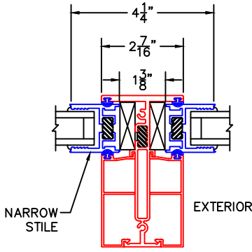
4 VERTICAL TDL W/NARROW STILE INSERT
