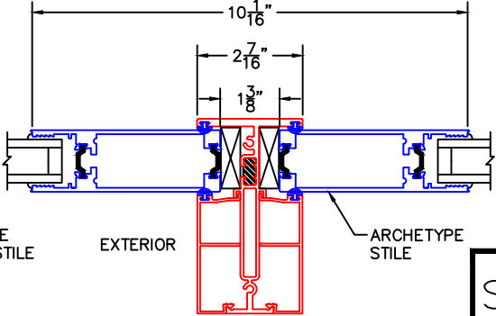
4B VERTICAL TDL W/ARCHETYPE STILE INSERT
