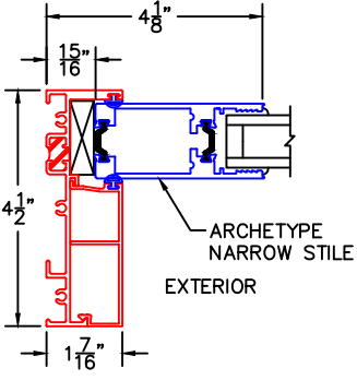
4A VERTICAL TDL W/ARCHETYPE NARROW STILE INSERT
