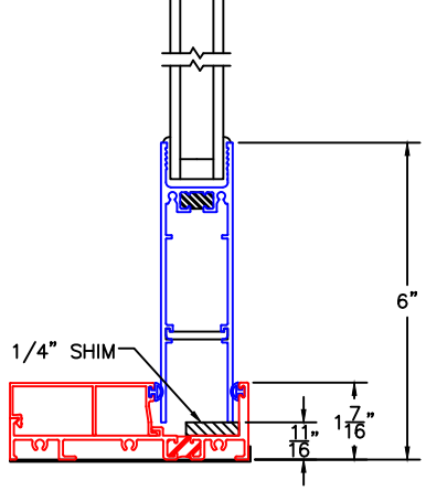
3A BLOCK JAMB W/ARCHETYPE NARROW STILE INSERT
