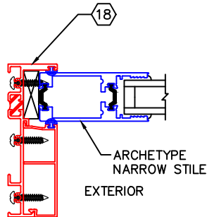
3A BLOCK JAMB W/ARCHETYPE NARROW STILE INSERT
