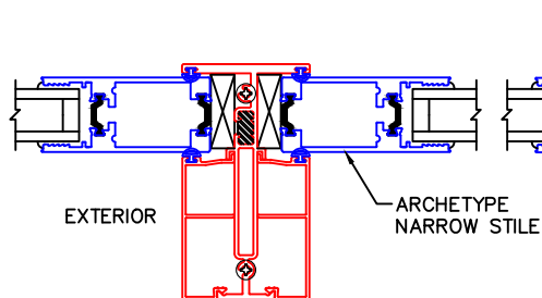
4A VERTICAL TDL W/ARCHETYPE NARROW STILE INSERT
