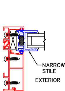
4A VERTICAL TDL W/ARCHETYPE NARROW STILE INSERT
