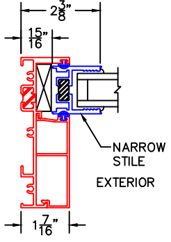
4A VERTICAL TDL W/ARCHETYPE NARROW STILE INSERT
