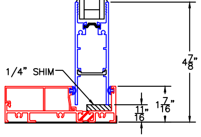
3A BLOCK JAMB W/ARCHETYPE NARROW STILE INSERT
