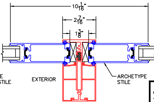
4B VERTICAL TDL W/ARCHETYPE STILE INSERT
