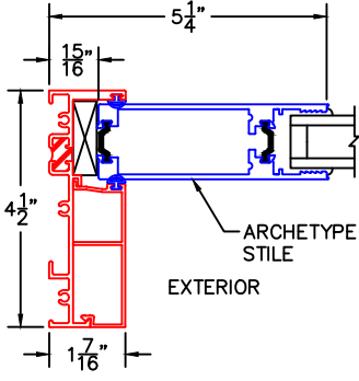
4B VERTICAL TDL W/ARCHETYPE STILE INSERT
