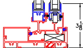
8 BLOCK SILL W/ SILL PAN
