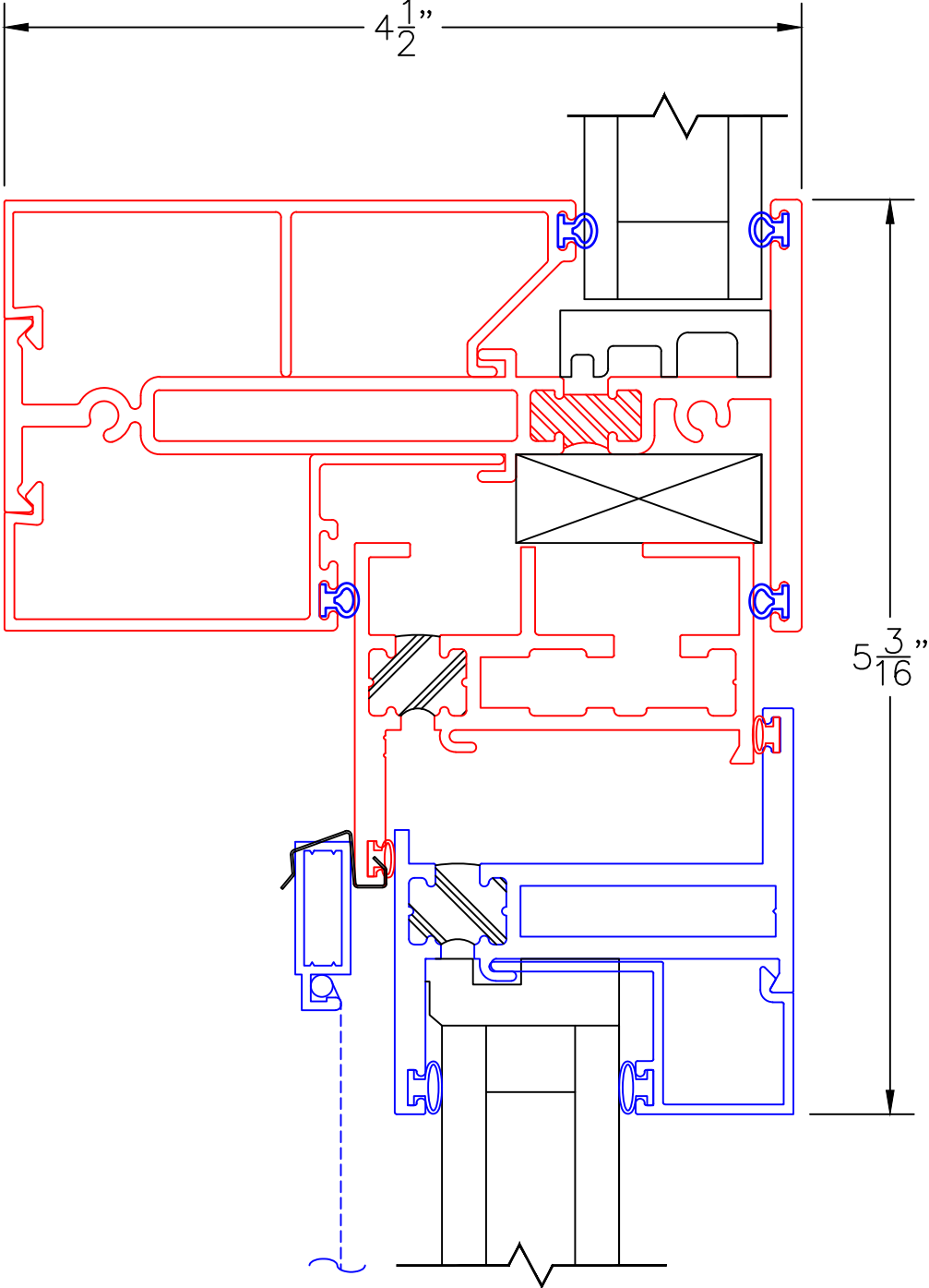
3800-T 1" GLAZING OVER 250-T HOPPER INSERT
