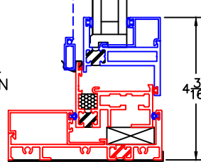
6 BLOCK SILL W/ SILL PAN
