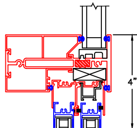
7 HORIZONTAL TDL
