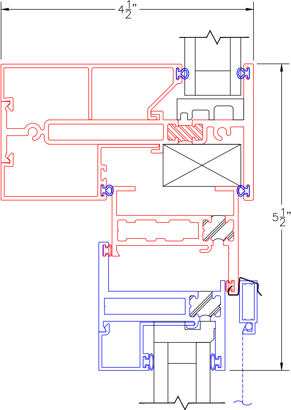
3800-T 1" GLAZING OVER 250-T CASEMENT INSERT
