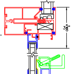
5 HORIZONTAL TDL
