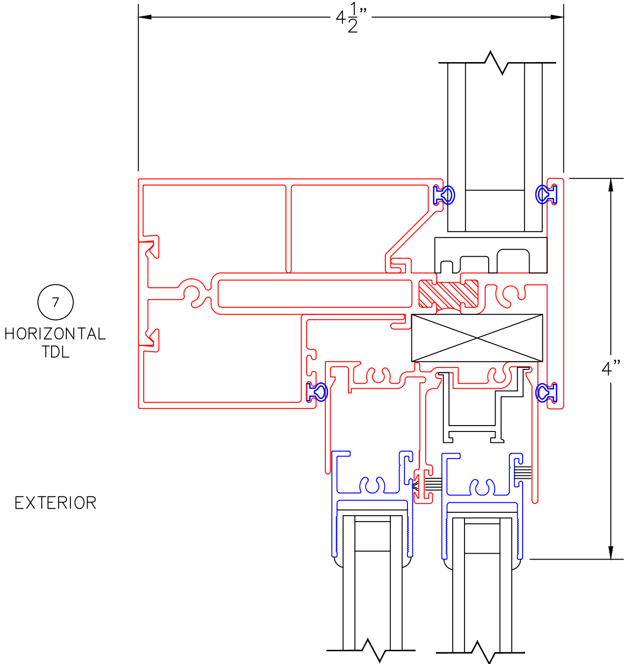
3800-T 1" GLAZING OVER 250 5\8" GLAZING XO SLIDER INSERT
