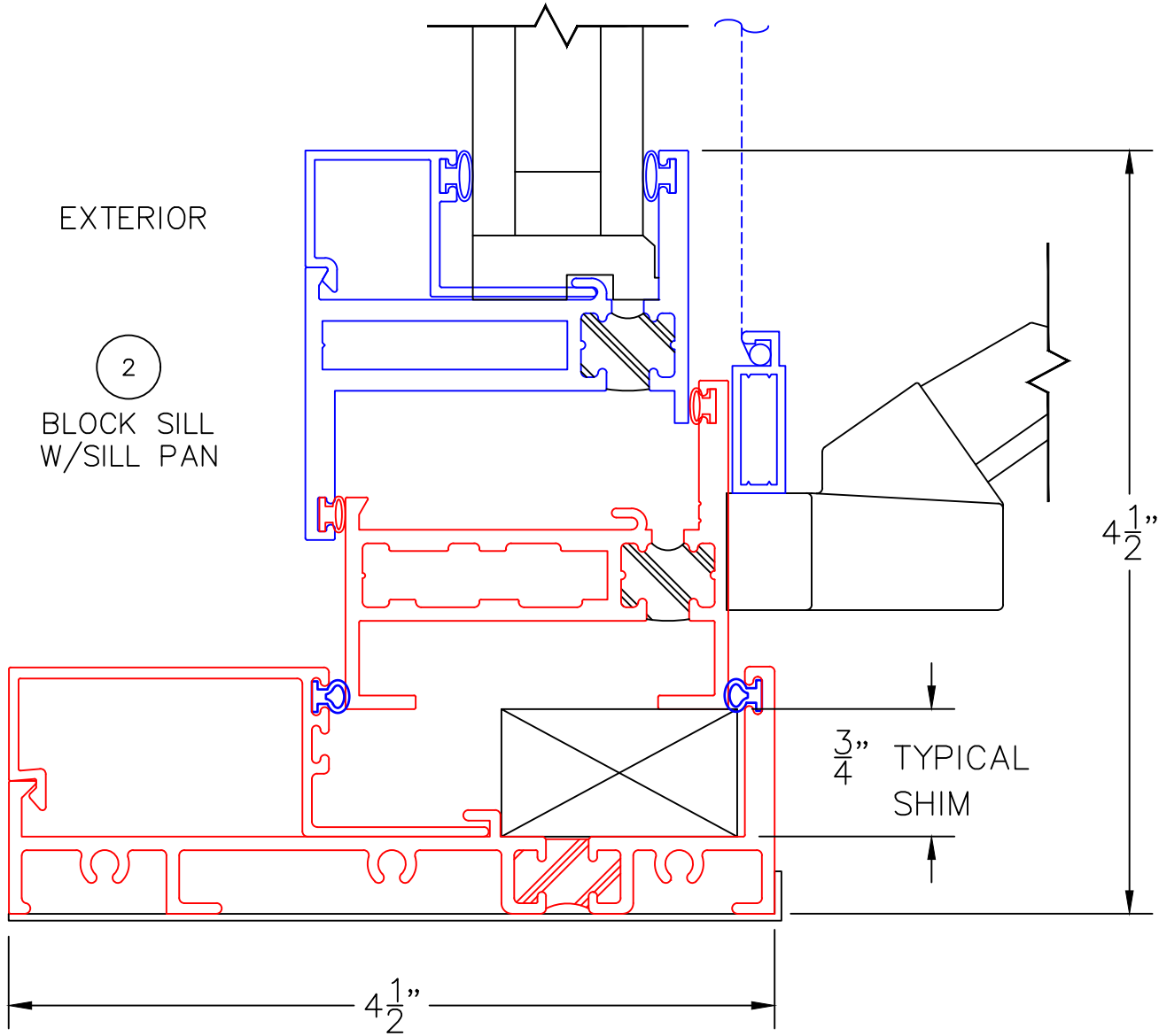
3800-T SILL WITH 250-T CASEMENT/AWNING INSERT
