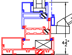
2 BLOCK SILL W/ SILL PAN
