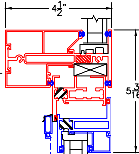
3 HORIZONTAL TDL
