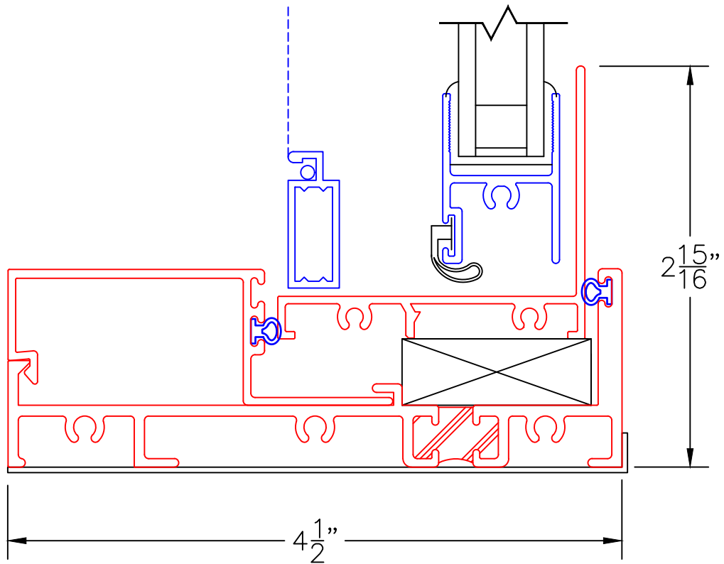
3800-T SILL WITH 250 SINGLE HUNG INSERT
