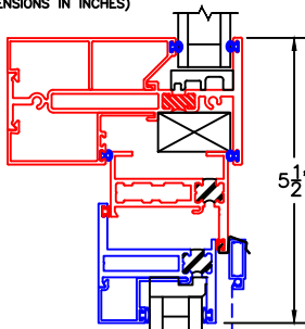
1 HORIZONTAL TDL
