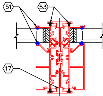
EXTERNAL "I" THERMALLY-BROKEN JAMB MULLION
