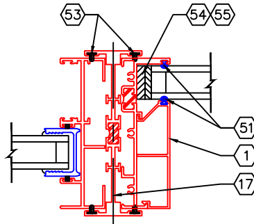
EXTERNAL "I" THERMALLY-BROKEN JAMB MULLION
