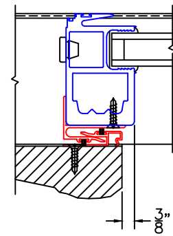
⑤ J-POST POCKET INTERLOCKER WITH REVERSE HP INTERLOCKER
