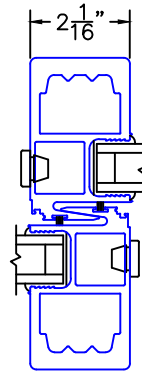
② HP INTERLOCKERS (BOTH)
