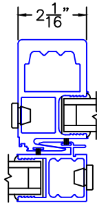
① HP INTERLOCKERS (STD)
