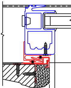
③ 2-PIECE POCKET INTERLOCKER WITH REVERSE HP INTERLOCKER
