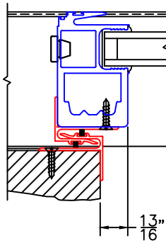
④ L-TYPE POCKET INTERLOCKER WITH REVERSE HP INTERLOCKER
