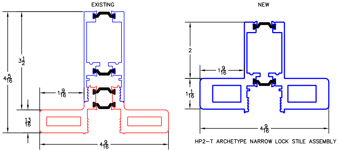
ARCHETYPE NARROW LOCK STILE ASSEMBLY WITH HP2-T ADAPTOR
