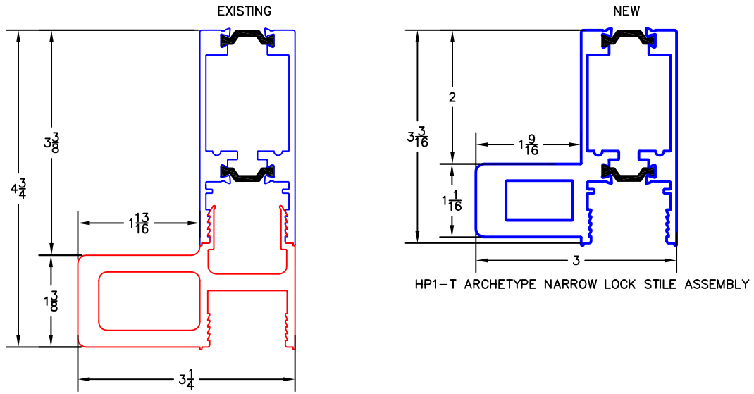
ARCHETYPE NARROW LOCK STILE ASSEMBLY WITH HP1 ADAPTOR
