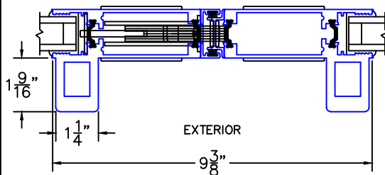
HP2-T ARCHETYPE NARROW MEETING STILES
