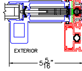
*HP2-T ARCHETYPE NARROW LOCK STILE
