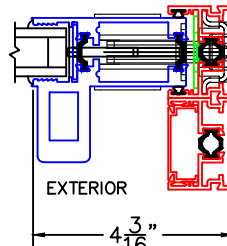
**HP1-T ARCHETYPE NARROW LOCK STILE
