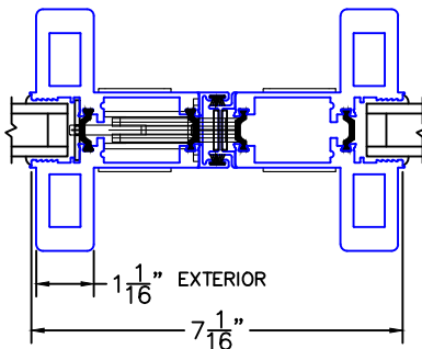
HP2-T ARCHETYPE NARROW MEETING STILES
