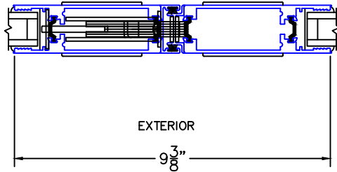
HP1-T ARCHETYPE MEETING STILES
