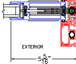
HP1-T ARCHETYPE LOCK STILE
