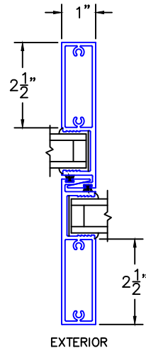
***NARROW HP INTERLOCKERS (BOTH SIDES)
