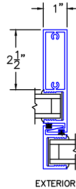
***NARROW HP INTERLOCKERS (INTERIOR SHOWN)
