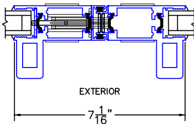
HP1-T ARCHETYPE NARROW MEETING STILES
