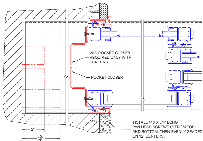
Figure 13: Head Bumper
