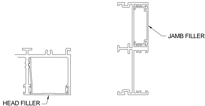
Figure 21: Head Filler
