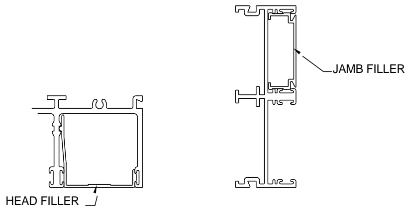
Figure 21: Head Filler
