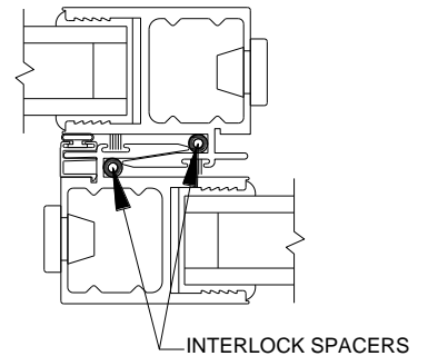
Figure 19: Proper Engagement of Interlockers
