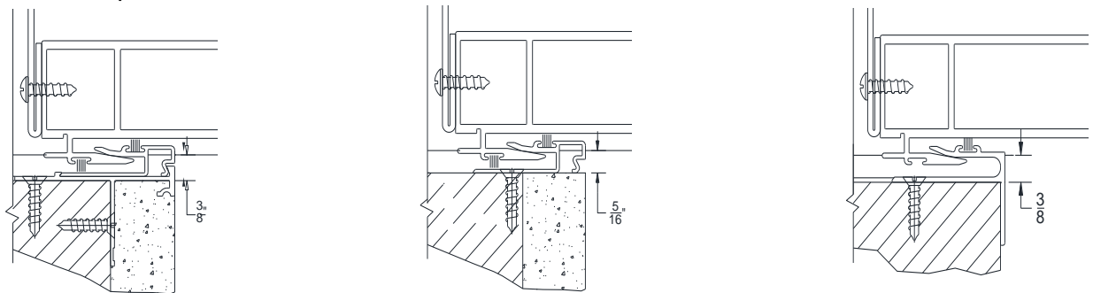
2 Piece Pocket Interlocker (Standard on 3050)
