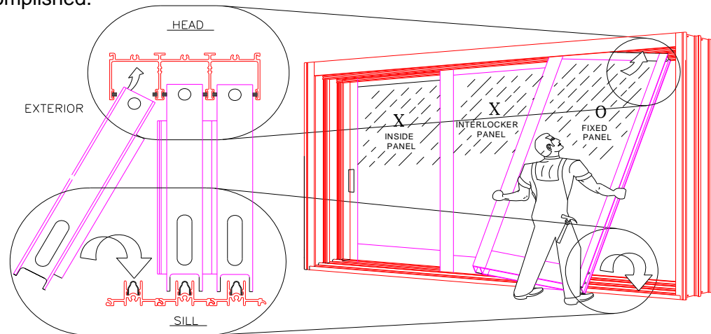
Figure 17: Panel Installation
