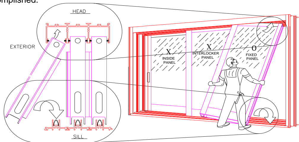
Figure 17: Panel Installation
