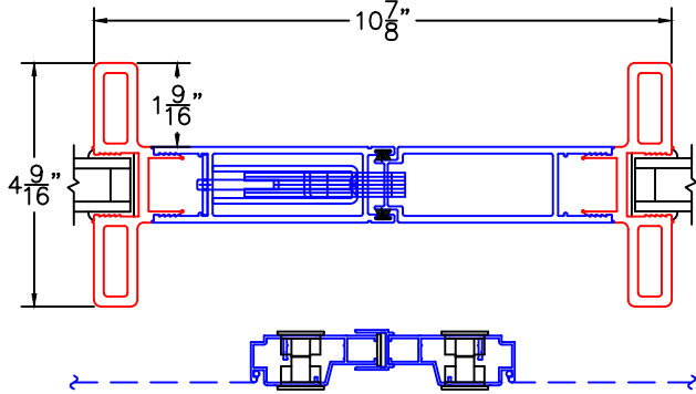
ARCHETYPE MEETING STILES WITH HP2 ADAPTERS
