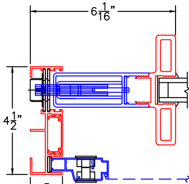
ARCHETYPE LOCK STILE WITH HP2 ADAPTER
