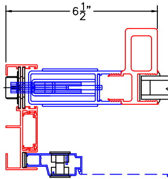
ARCHETYPE LOCK STILE WITH HP1 ADAPTER
