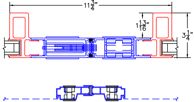
ARCHETYPE MEETING STILES WITH HP1 ADAPTERS
