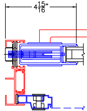
ARCHETYPE LOCK STILE WITH LEVER
