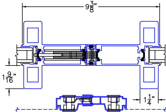
HP2-T ARCHETYPE MEETING STILES
