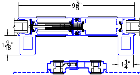
HP1-T ARCHETYPE MEETING STILES
