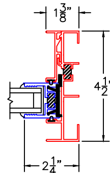
FIXED JAMB WITH O-PANEL SNAP-IN (BLOCK ONLY)
