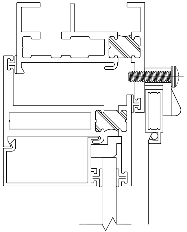
EXISTING PLASTIC SCREEN CLIP
