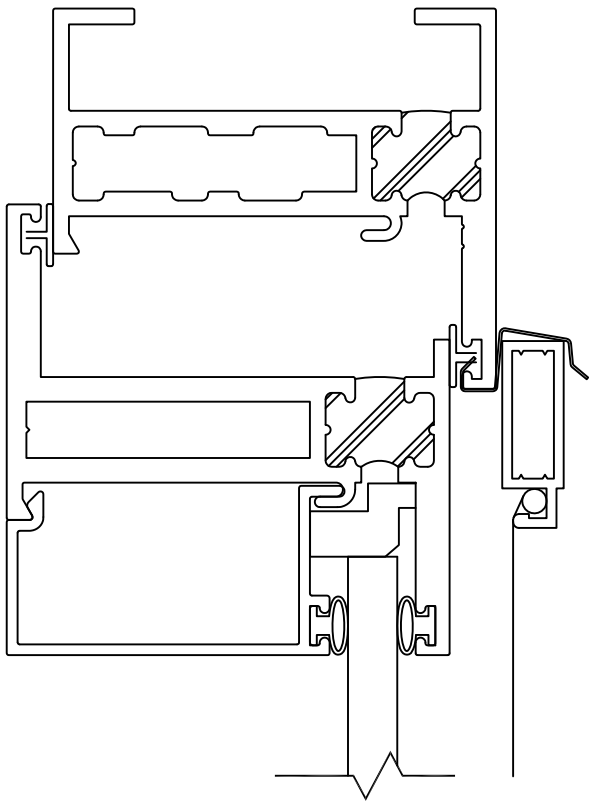
NEW STAINLESS STEEL SCREEN CLIP
